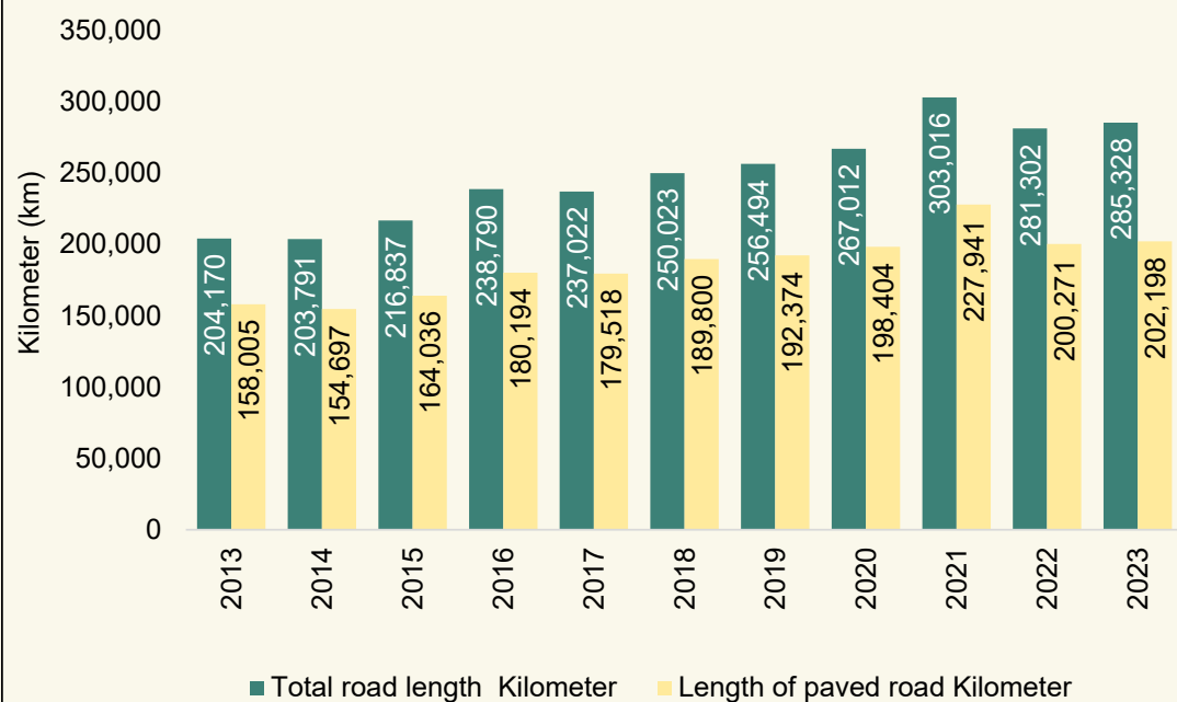
Chart 1.1 Length of Road, 2013 - 2023
